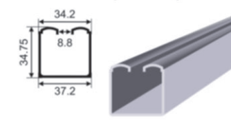
SLIDING DOOR CHANNEL DC-452
