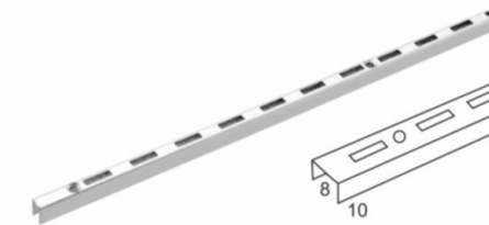
BRACKET CHANNEL (SINGLE SLOT) DC-02
