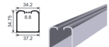
SLIDING DOOR CHANNEL WITH PLASTIC DC-451
