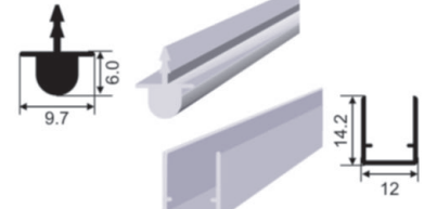
CABINET SLIDING CHANNEL 'A' DC-255
