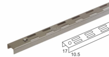
BRACKET CHANNEL (Double Slot Broad) DC-05
