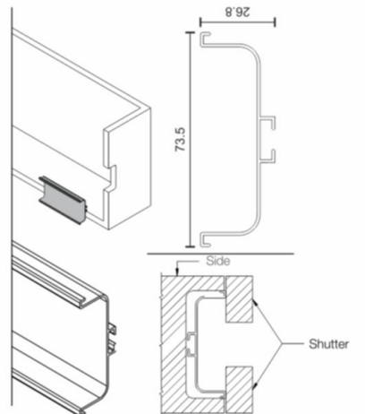
C-GOLA PROFILE DC-1111
