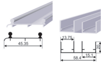
WARDROBE SLIDING CHANNEL (Double Track) DC-246
