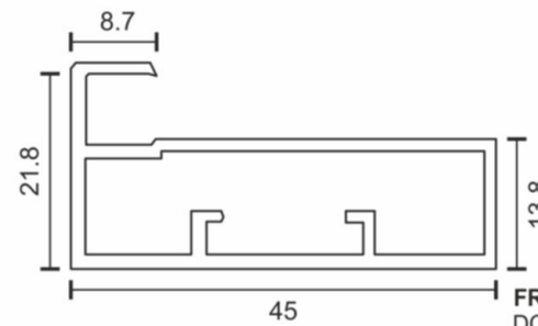
FRAME E- PROFILE DC-1101
