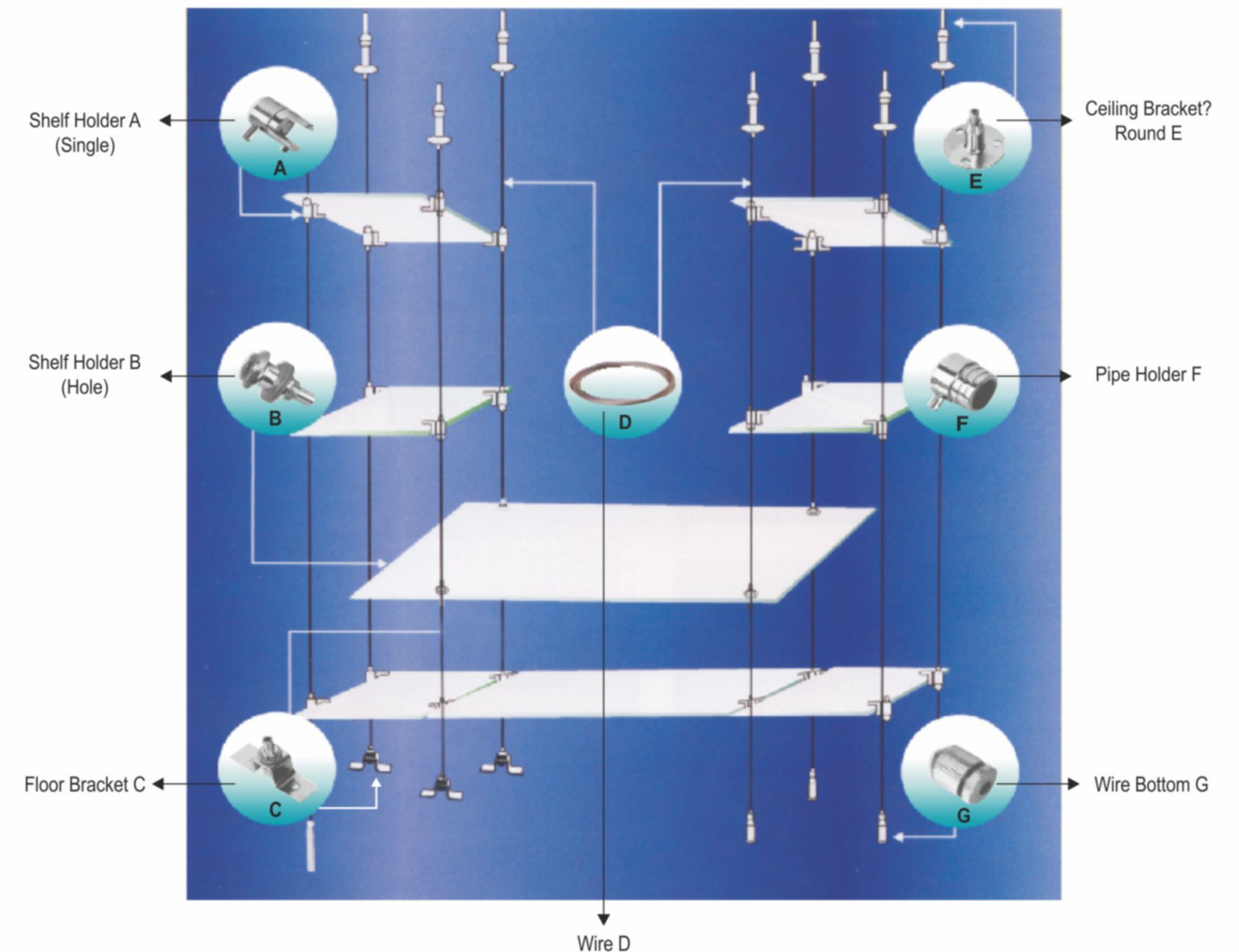
FRAMELESS WIRE DISPLAY SYSTEM DC-218
