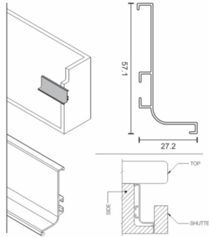
J-GOLA PROFILE DC-1110
