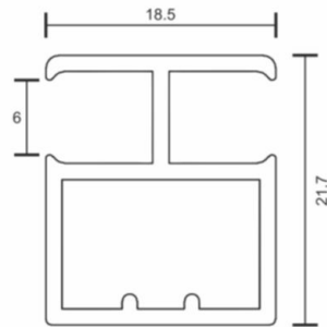
DIVIDER PROFILE DC-1120
