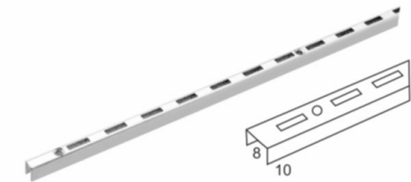
BRACKET CHANNEL (SINGLE SLOT) DC-03
