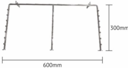
E-TYPE CHANNEL HANGER STAND DC-19
