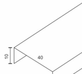
U-TYPE CHANNEL (40mm) DC-1152
