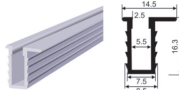
HI-TECH CABINET SLIDING CHANNEL DC-248
